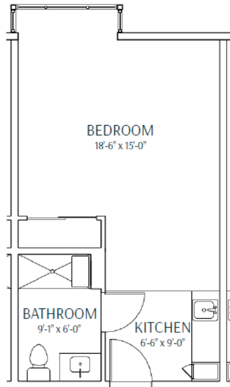
STUDIO - TYPE D 375 Square Feet
