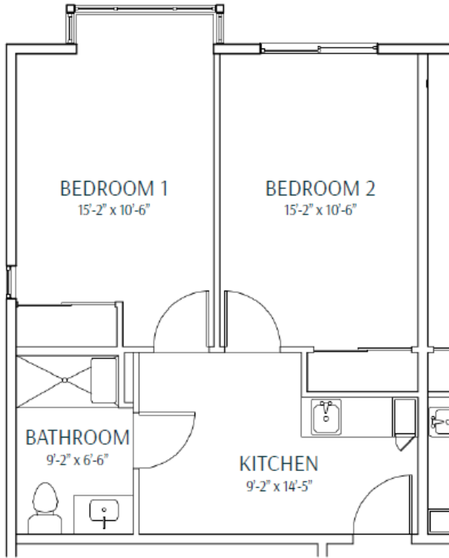
SHARED SUITE - TYPE A1 525 Square Feet 364 SQFT/RESIDENT
